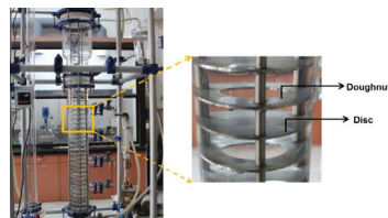
Liquid – Liquid Extraction Column
